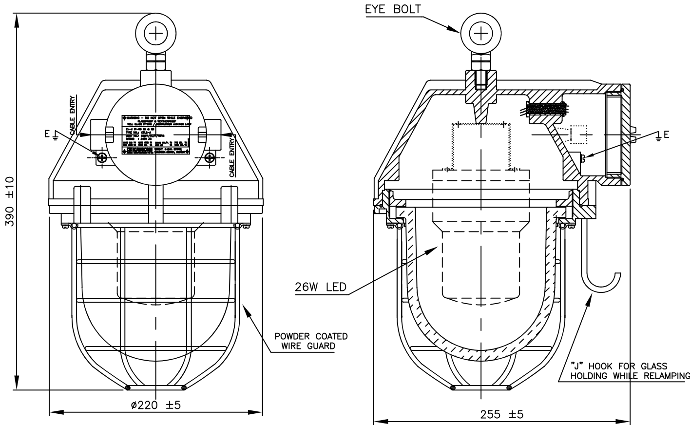
SPECIFICATION FOR 26W LED
